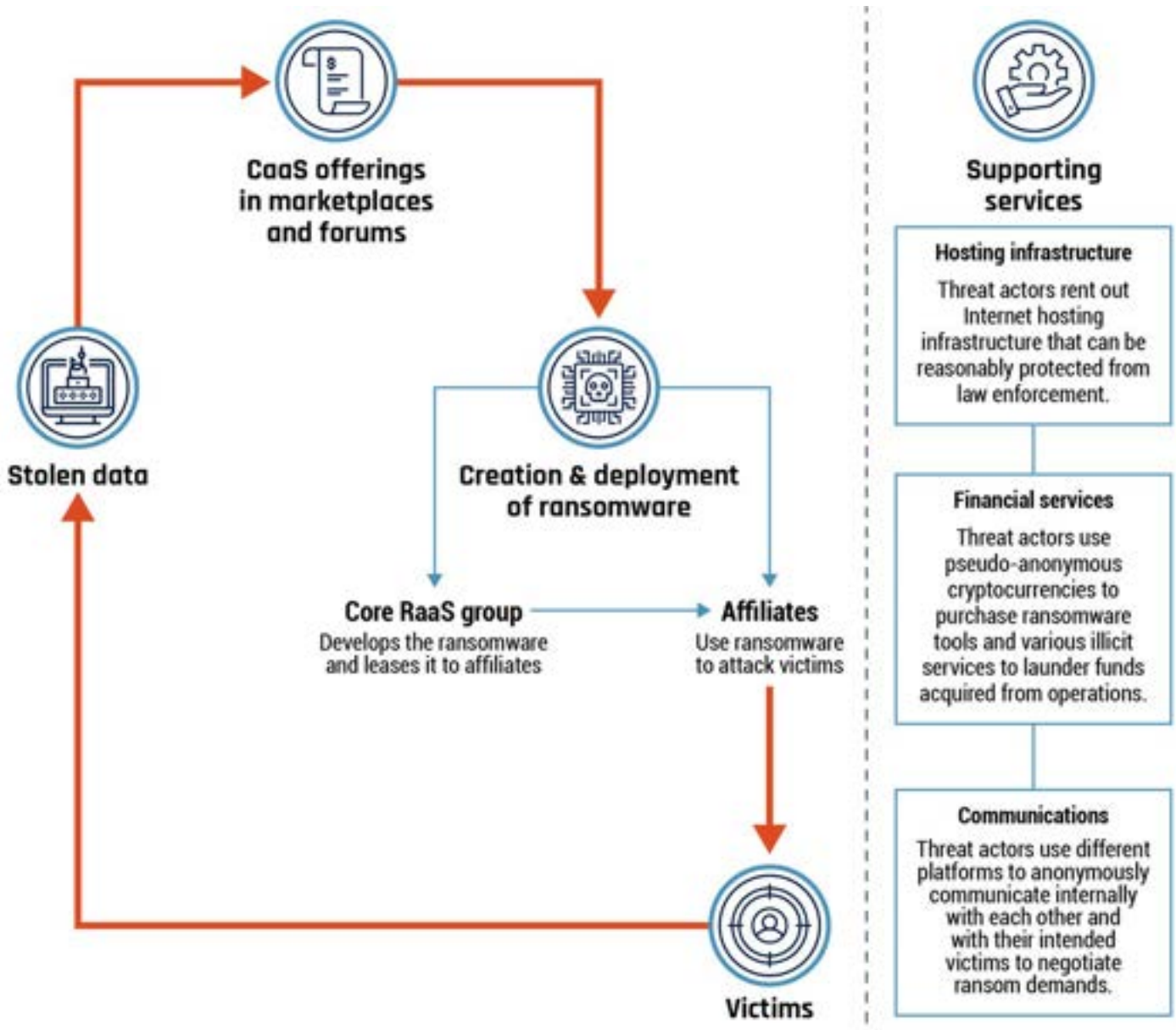
Figure 10: RaaS ecosystem
